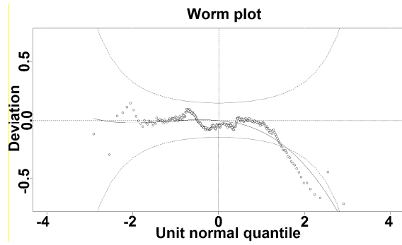
Figure W2 – Tests of normality of residuals for the beta distribution (logit link)
