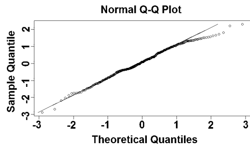
Figure W2 – Tests of normality of residuals for the beta distribution (logit link)
