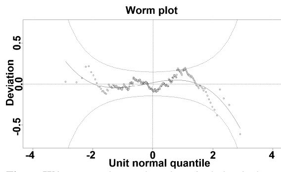
Figure W1 – Tests of normality of residuals for the linear model
